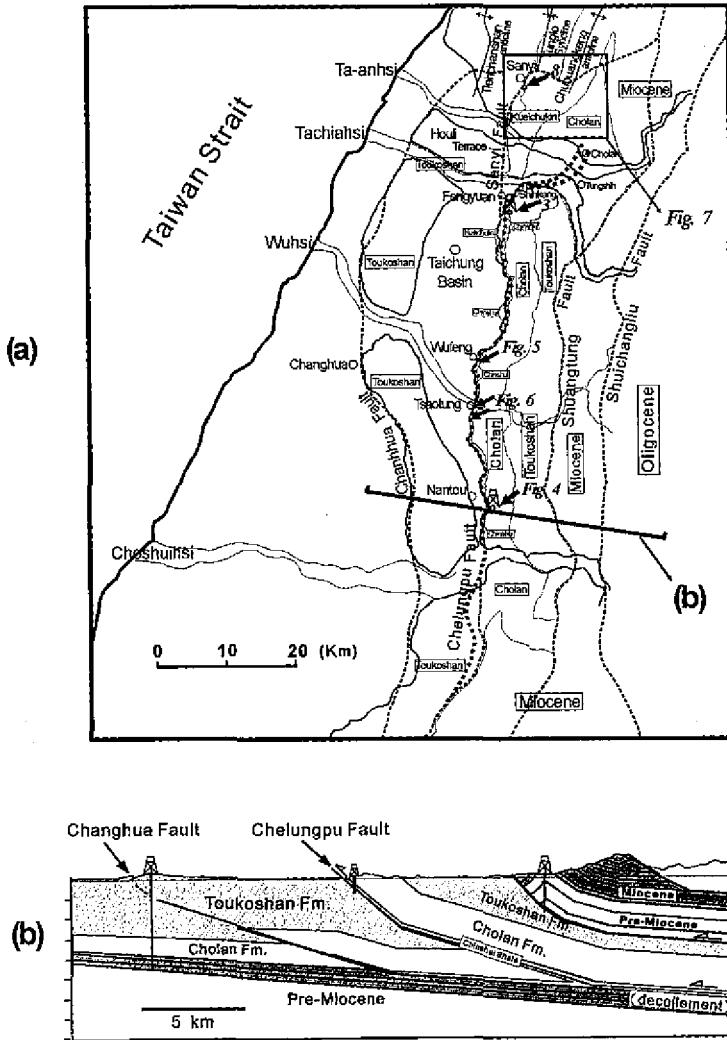
Fig. 1. (a) A simplified geological map of the area surrounding the Chelungpu fault and (b) a thin-skinned thrust model proposed by Suppe et al. (2000). Four sequential faults (from west to east) separate the structures of the Pleistocene (Toukoshan Formation), the Pliocene (Cholan, Chinshui, and Kueichulin Formations), the Miocene, and the Oligocene. It is noticed that the Changhai fault (the most western one) bends to the east at its northern end, north of the Ta-anhsi river. The Chelungpu fault follows the boundary between the foothills on the east and the Taichung basin on the west. The Sanyi fault extends from the Chelungpu fault, near Fengyuan, and then goes straight north, but also bends to the east near Sanyi. The arrows point out the numbered places to be discussed in the next figures.
