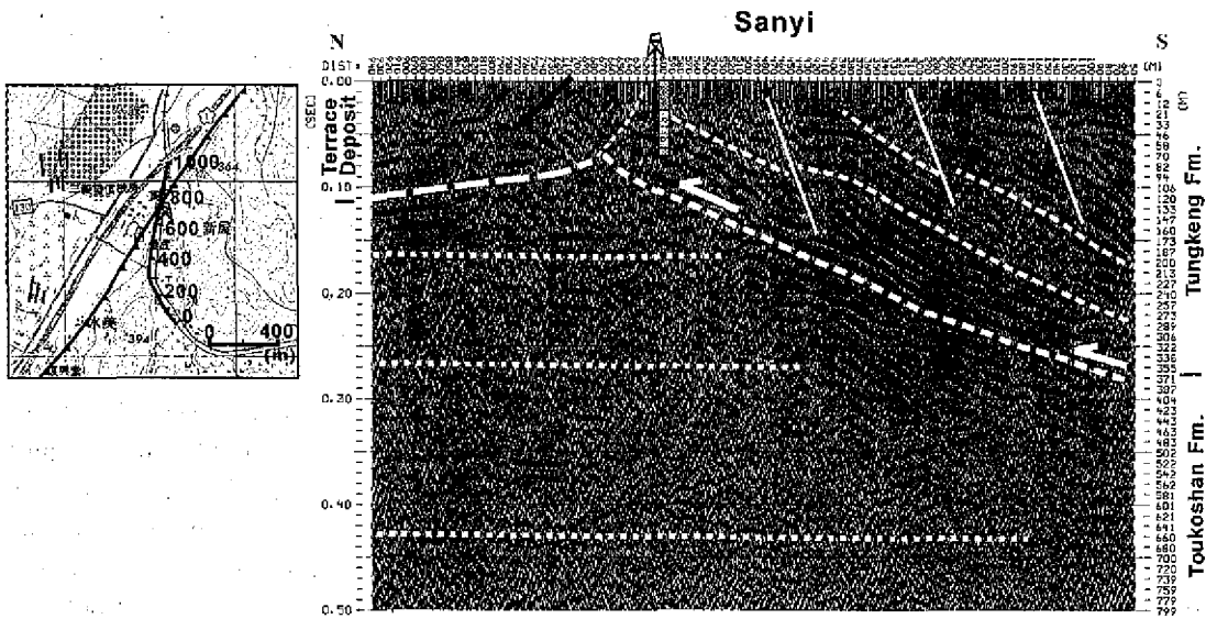
Fig. 8. A seismic reflection section crossing the Sanyi fault. The survey site was at the south of the town of Sanyi (Fig. 1a). The Sanyi fault slides along the Tungkeng Formation which contains layers that dip to the southeast. The flat layers of the late Quaternary gravel deposits are visible on the lower-left part of the section. The upper-left corner (arrowed) has an odd westward dipping layer which can be explained as a terrace deposit. An 'eroded-toe' model is proposed to interpret this unusual structure.
