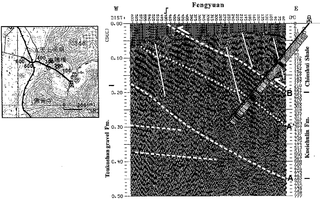
Fig. 3. A shallow reflection seismic section taken adjacent to the Fengyuan well at the northern portion of the Chelungpu fault. Most of the layers dip to the east, except the bottom one, which is flat. The surface rupturing caused by the earthquake is located at the 480 m position (shown by a step symbol). Symbol A represents the boundary between the Kueichulin Formation (inclined) and the late Quaternary gravel deposits (flat). Symbol B is located between the Kueichulin Formation and the Chinshui Shale (disturbed), which is supposed to be the fault surface of the earthquake. It is obvious that the B boundary can be connected to the place of surface rupture. There is a strong reflection boundary A' inside the Kueichulin Formation, which can also be tied to a fracture zone observed in the well. Fractures are indicated with slanted line segments, which are believed to have been caused by the faulting as it thrust upward along the layer boundary, causing fracturing at a 45° angle to the layer.
